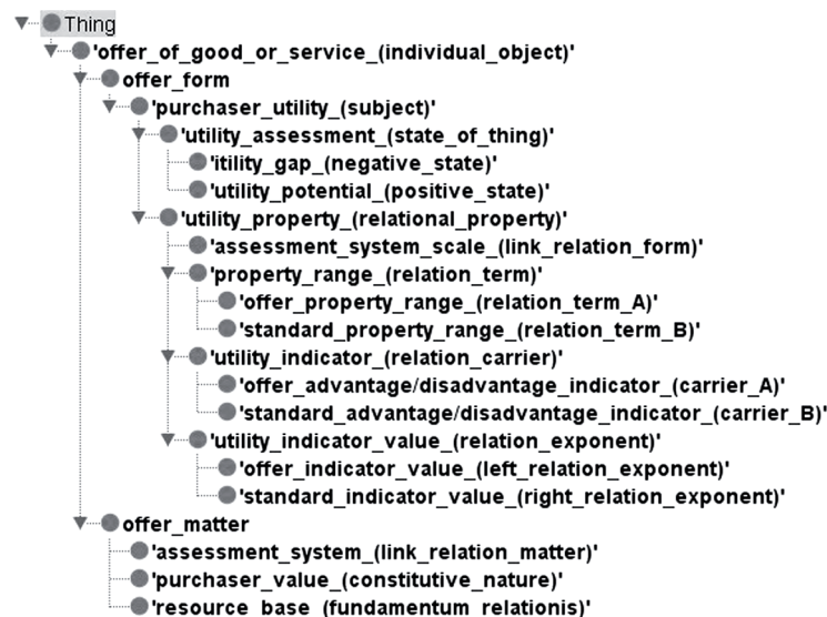
Fig. 4. A class (concept) diagram of ontology OOWU in the OWL language
